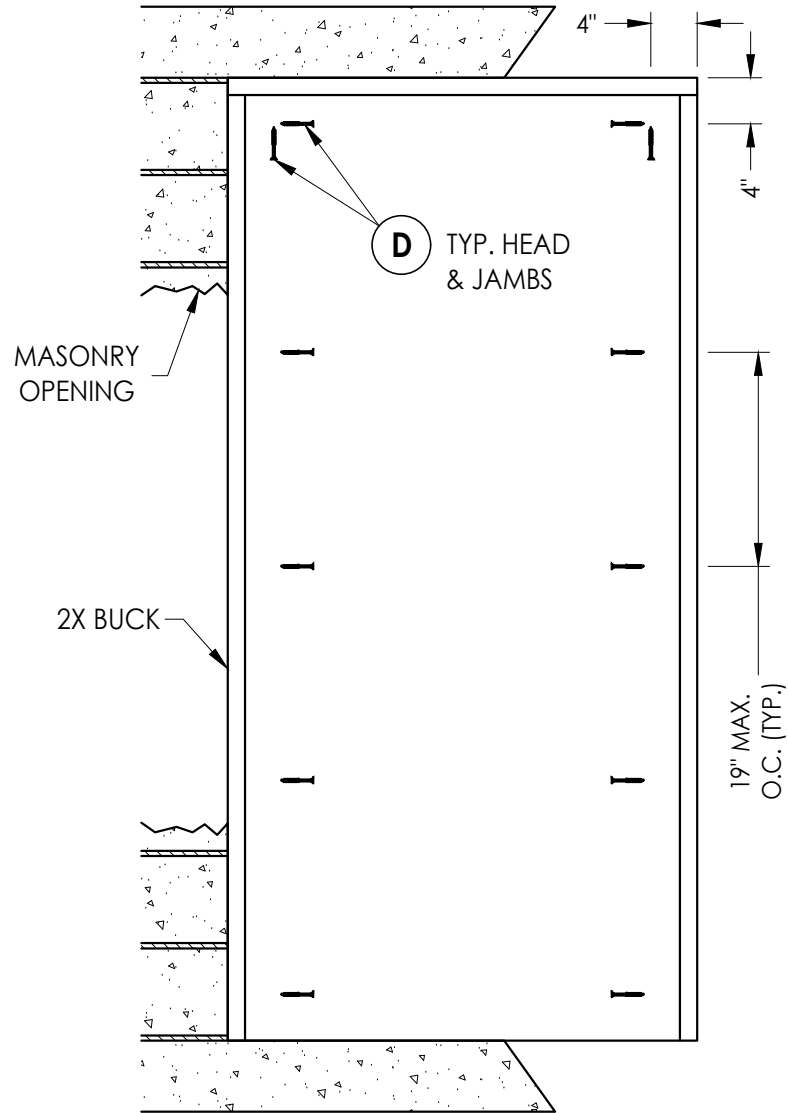
BUCK ANCHORING
