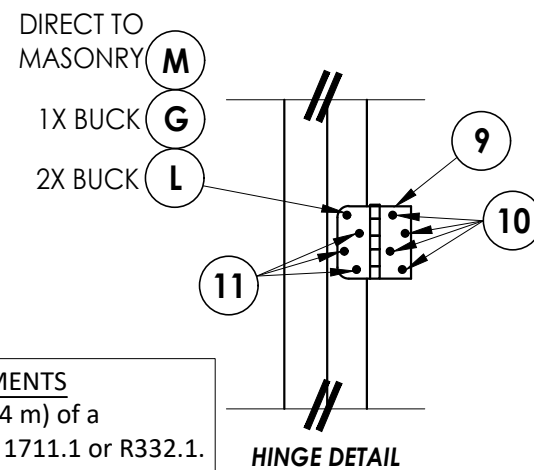
HINGE DETAIL
